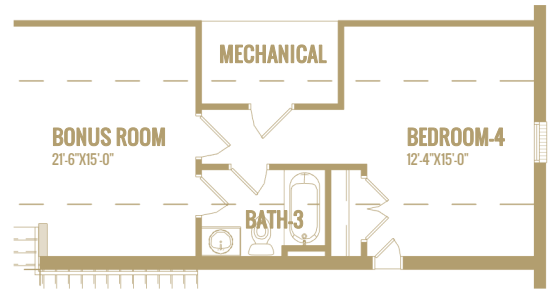
6 SECOND FLOOR LAYOUT 'B' (Adds 255 Sq.Ft.)
